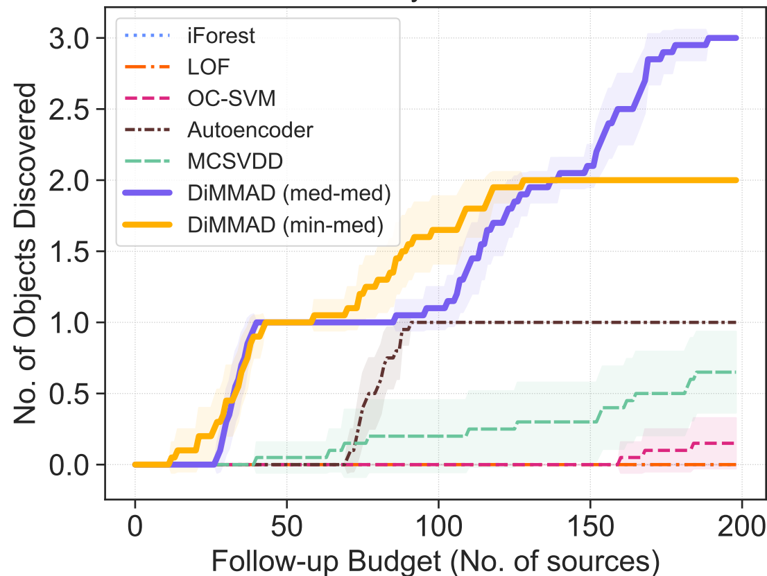
Anomaly: SL-SN1a
